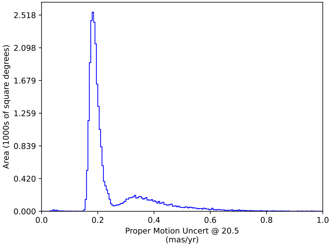
too_elab_r64_d2_ugrizy_v3.4_10yrs : Proper Motion Uncert @ 20.5
