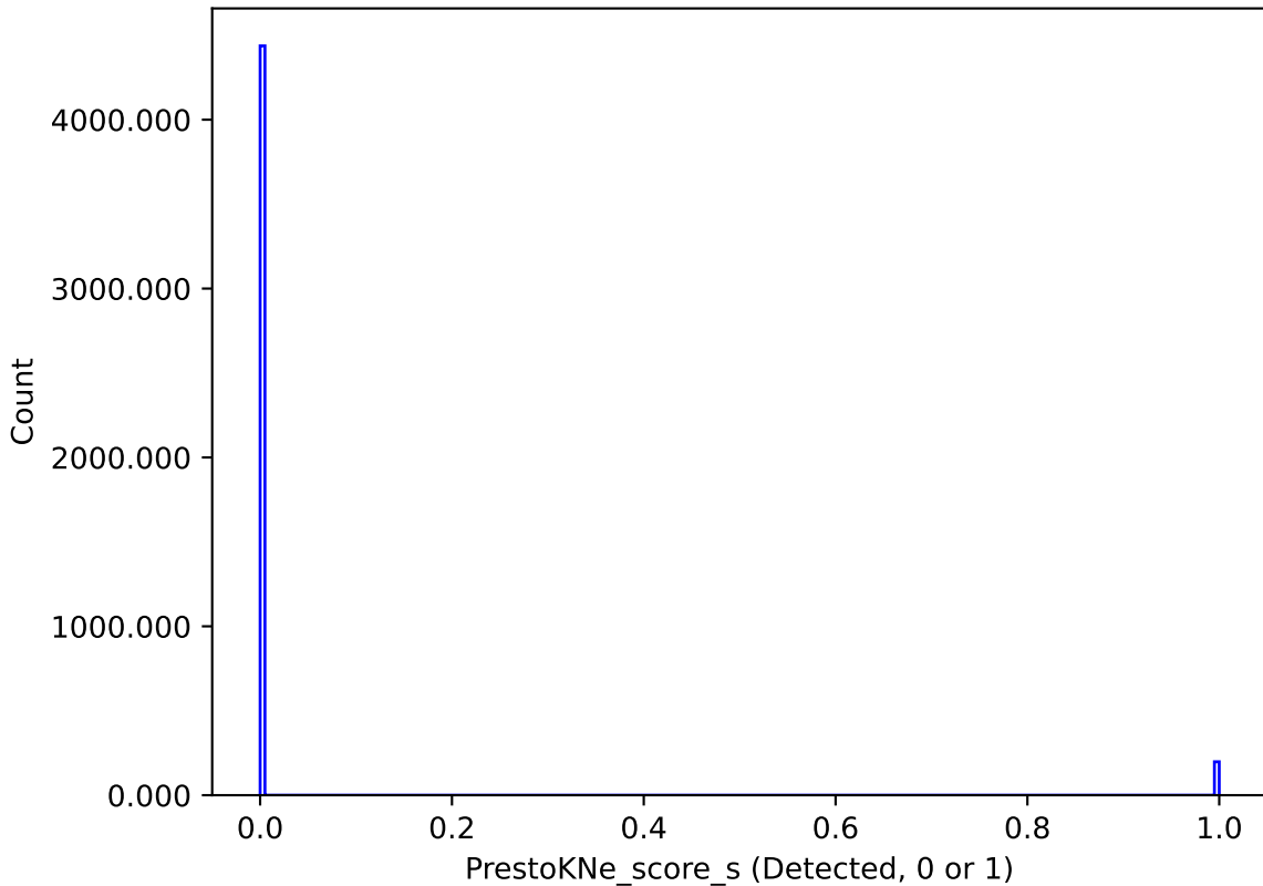
too_elab_r64_d2_ugrizy_v3.4_10yrs : PrestoKNe_score_s
