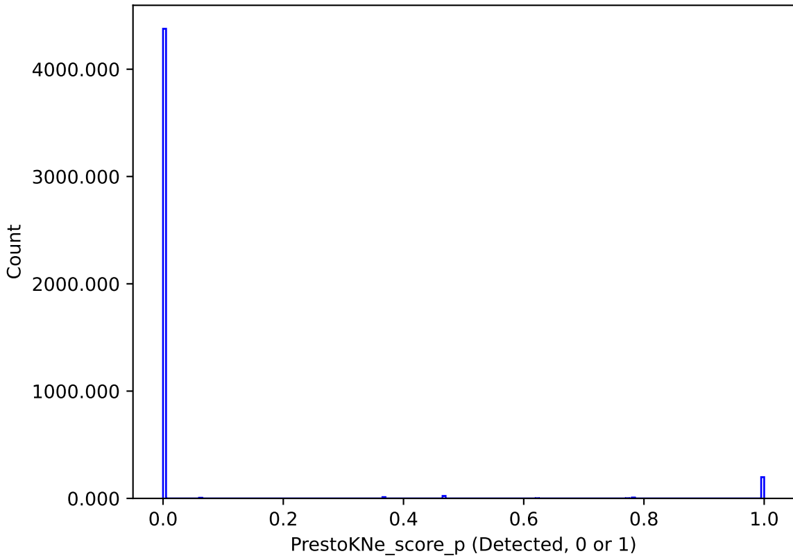
too_elab_r64_d2_ugrizy_v3.4_10yrs : PrestoKNe_score_p
