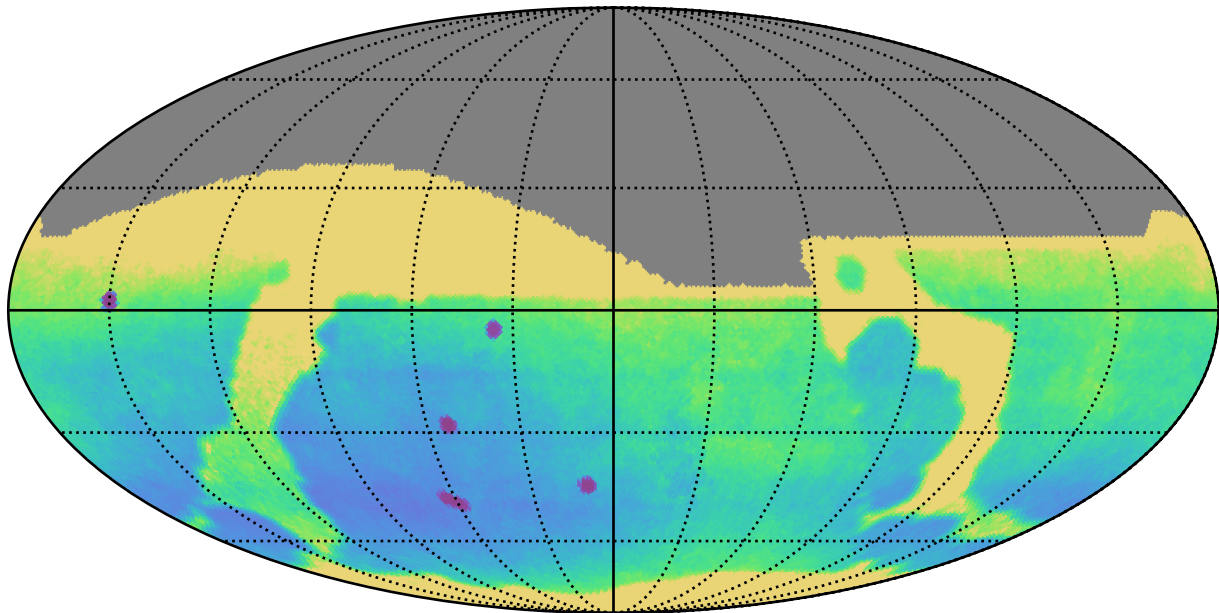
too_elab_r64_d2_ugrizy_v3.4_10yrs : Parallax Uncert @ 24.0
