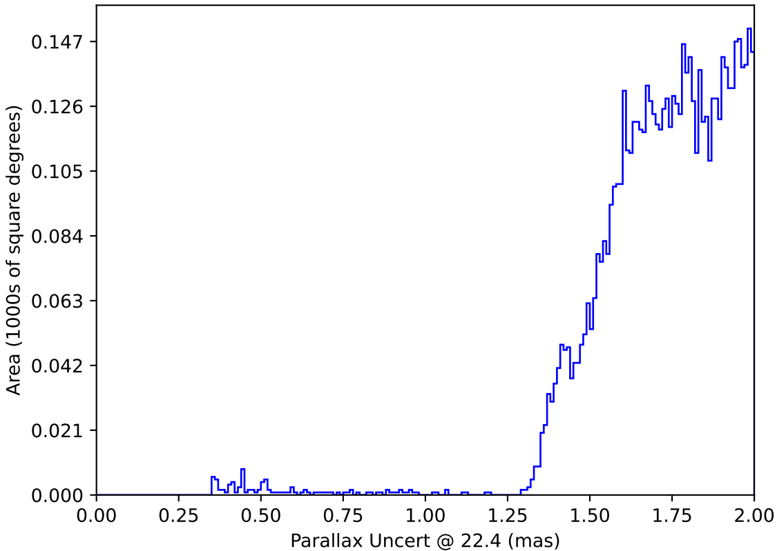
too_elab_r64_d2_ugrizy_v3.4_10yrs : Parallax Uncert @ 22.4
