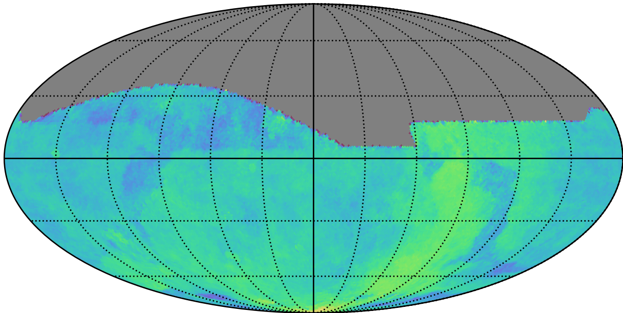
too_elab_r64_d2_ugrizy_v3.4_10yrs : Parallax Coverage @ 24.0
