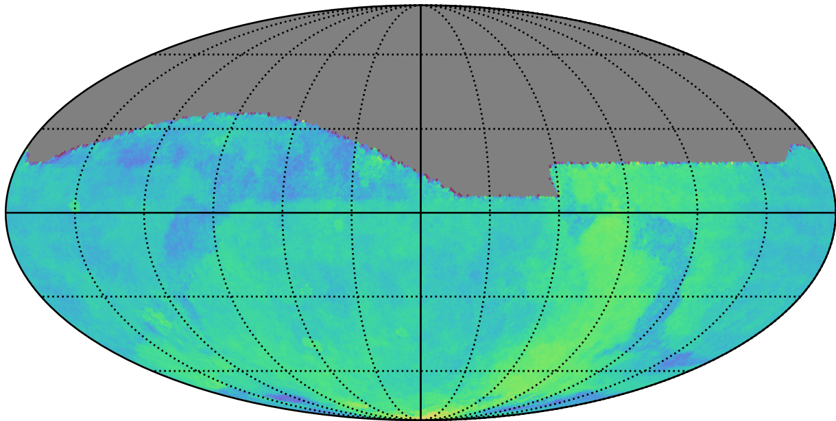
too_elab_r64_d2_ugrizy_v3.4_10yrs : Parallax Coverage @ 22.4
