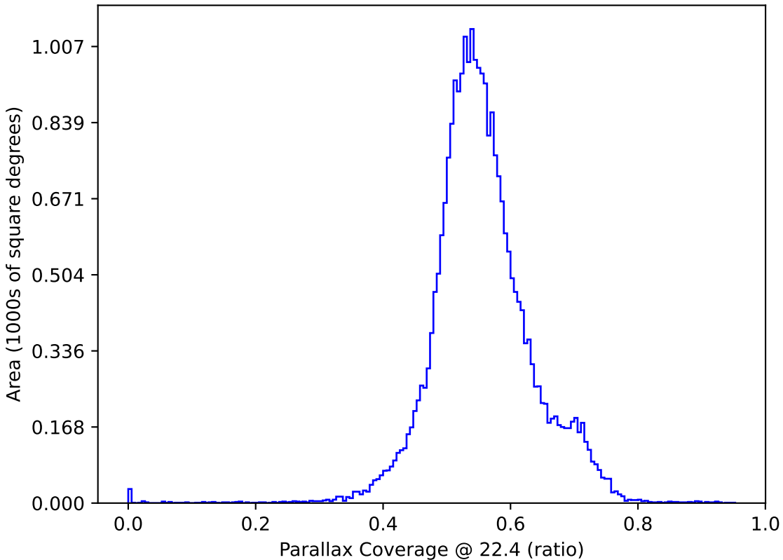
too_elab_r64_d2_ugrizy_v3.4_10yrs : Parallax Coverage @ 22.4
