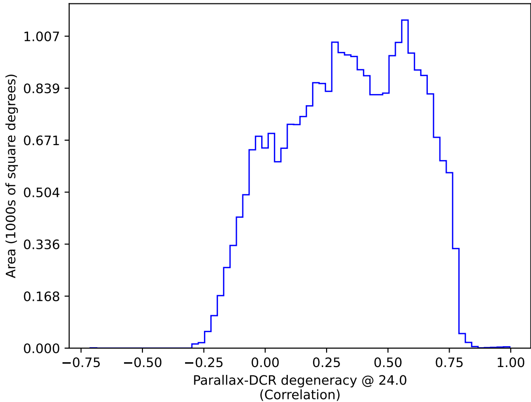
too_elab_r64_d2_ugrizy_v3.4_10yrs : Parallax-DCR degeneracy @ 24.0
