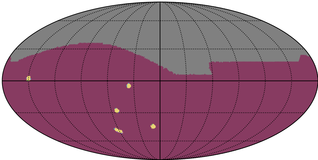
too_elab_r64_d2_ugrizy_v3.4_10yrs : NumberOfQuickRevisits
