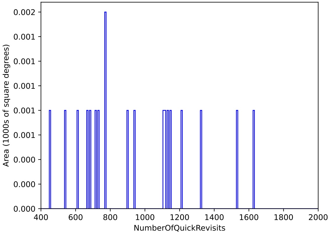
too_elab_r64_d2_ugrizy_v3.4_10yrs : NumberOfQuickRevisits
