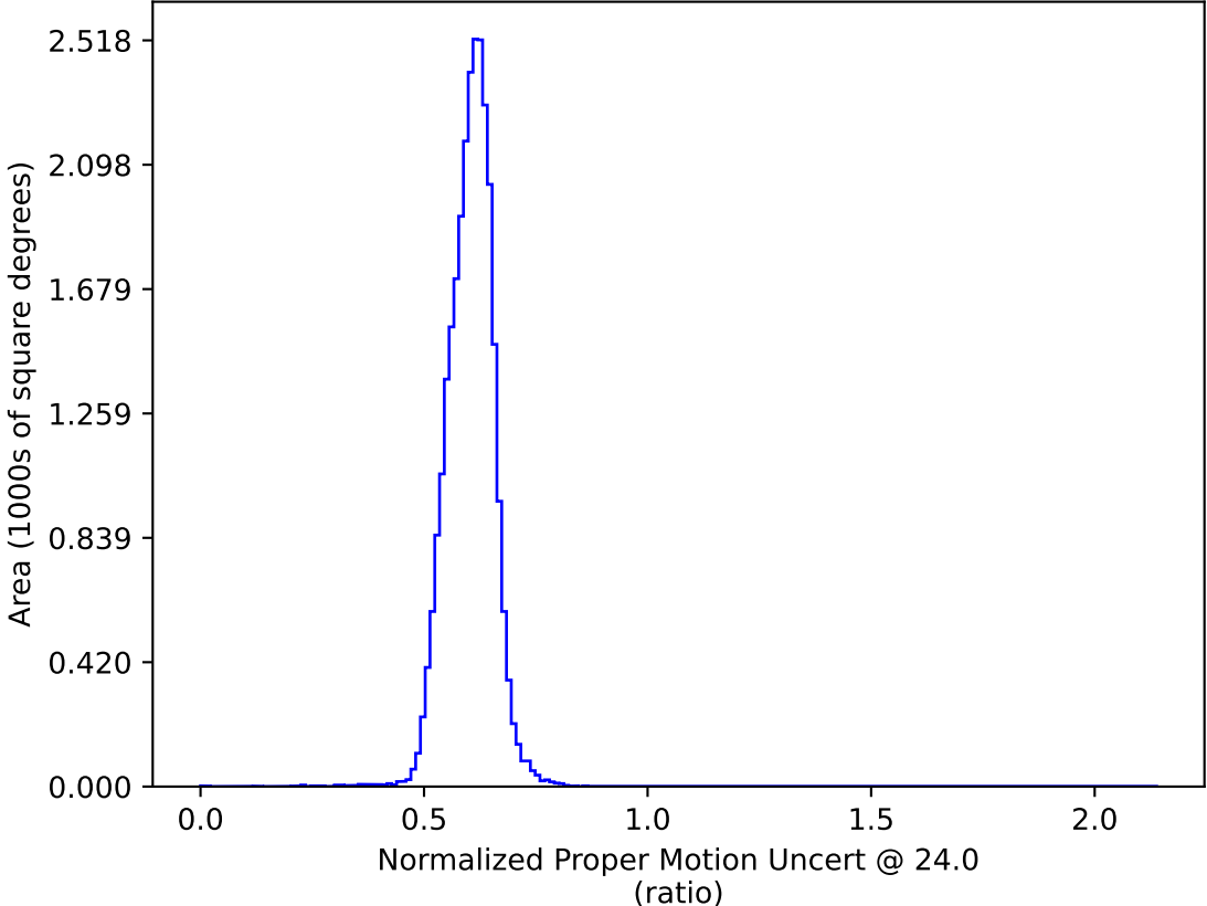
too_elab_r64_d2_ugrizy_v3.4_10yrs : Normalized Proper Motion Uncert @ 24.0
