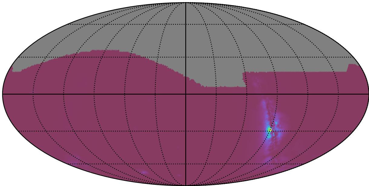
too_elab_r64_d2_ugrizy_v3.4_10yrs : NlcPoints
