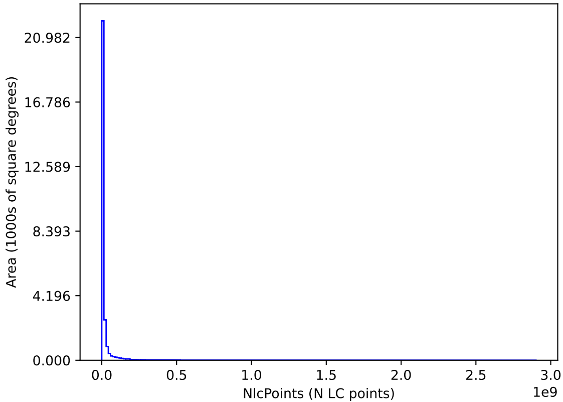
too_elab_r64_d2_ugrizy_v3.4_10yrs : NlcPoints
