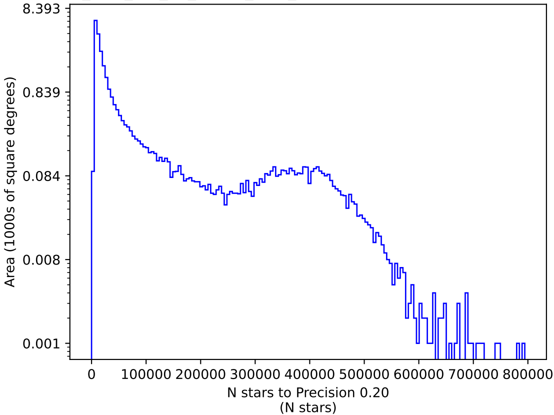
too_elab_r64_d2_ugrizy_v3.4_10yrs z: N stars to Precision 0.20
