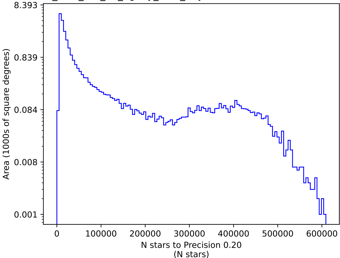
too_elab_r64_d2_ugrizy_v3.4_10yrs i: N stars to Precision 0.20
