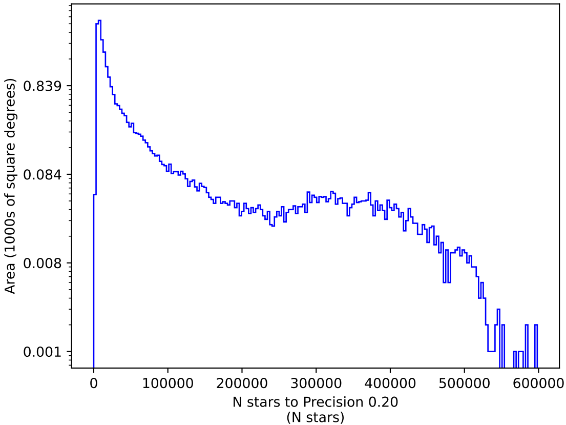
too_elab_r64_d2_ugrizy_v3.4_10yrs g: N stars to Precision 0.20
