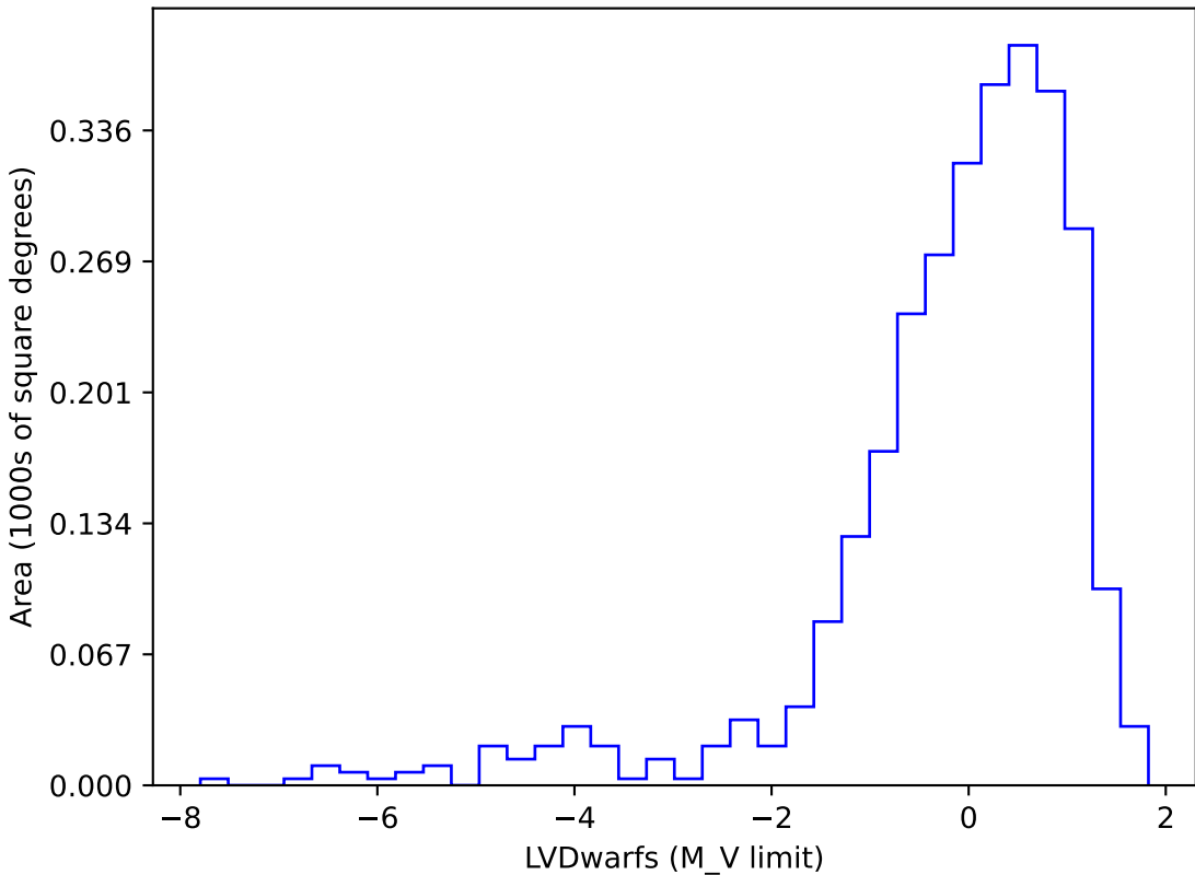
too_elab_r64_d2_ugrizy_v3.4_10yrs gi SCP: LVDwarfs
