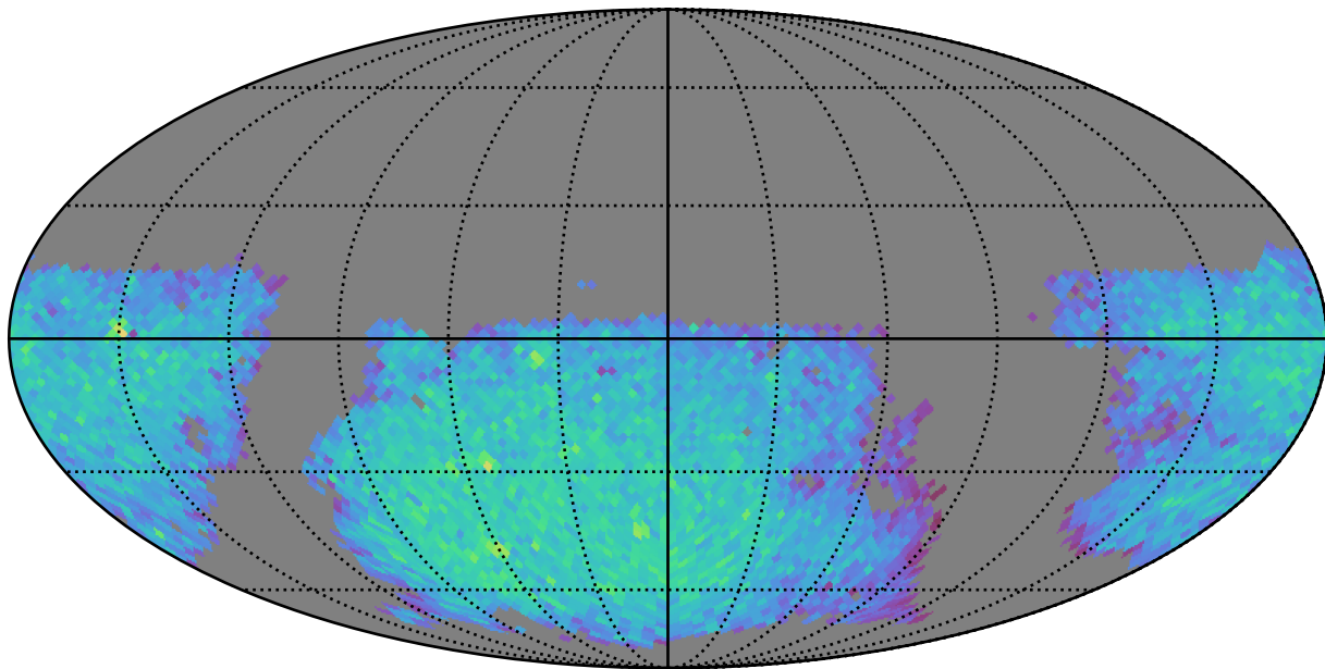
too_elab_r64_d2_ugrizy_v3.4_10yrs gi: LVDwarfs
