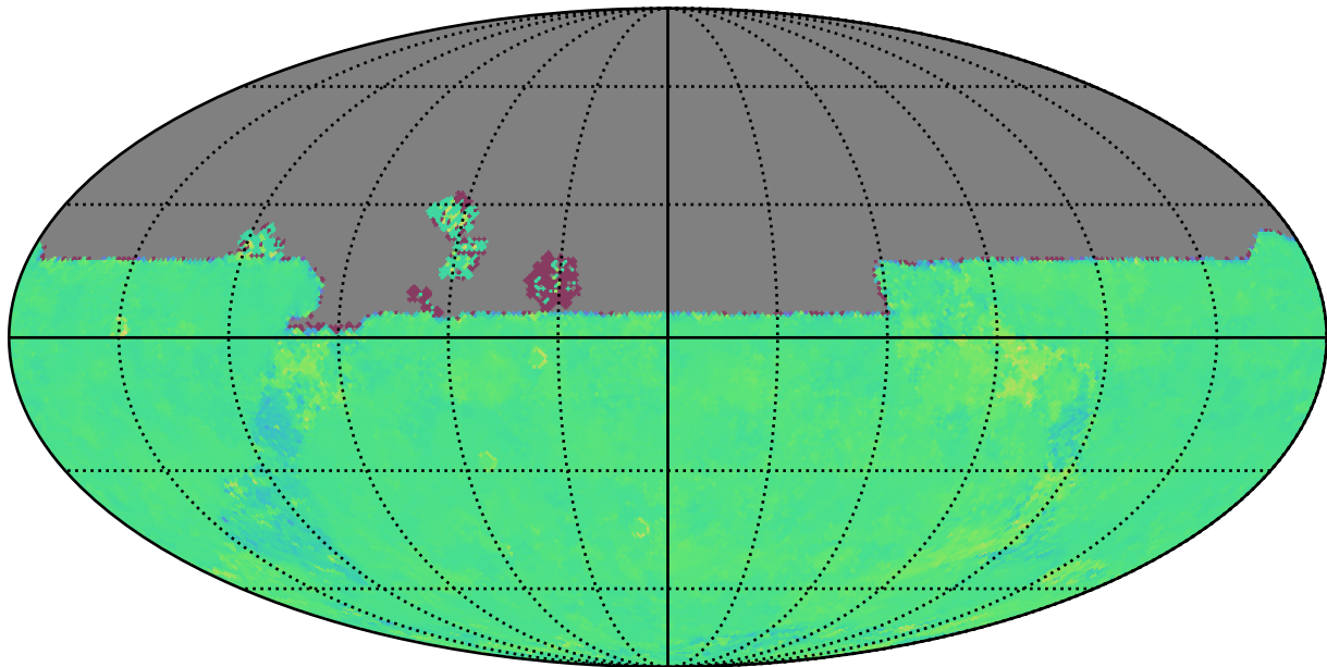
too_elab_r64_d2_ugrizy_v3.4_10yrs u: Kuiper rotTelPos
