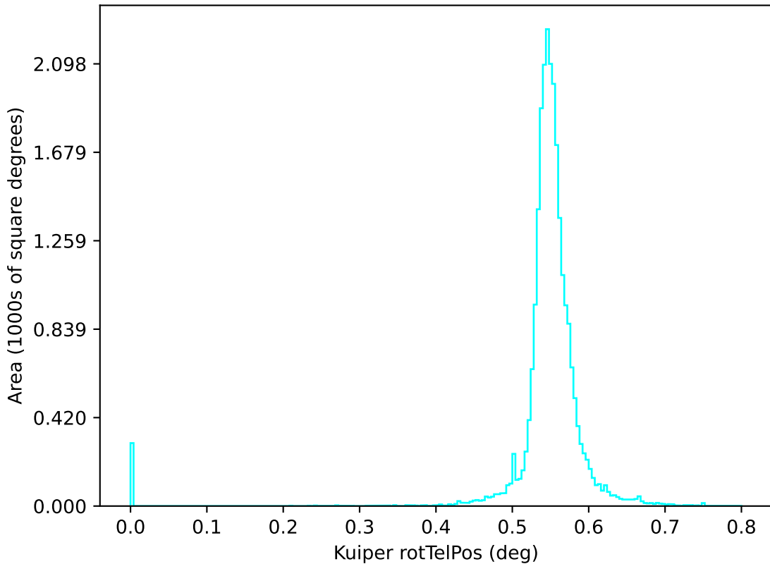
too_elab_r64_d2_ugrizy_v3.4_10yrs u: Kuiper rotTelPos
