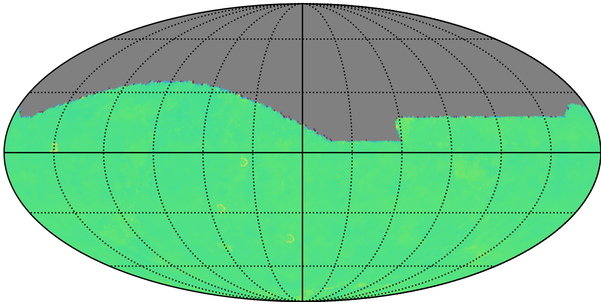
too_elab_r64_d2_ugrizy_v3.4_10yrs r: Kuiper rotTelPos
