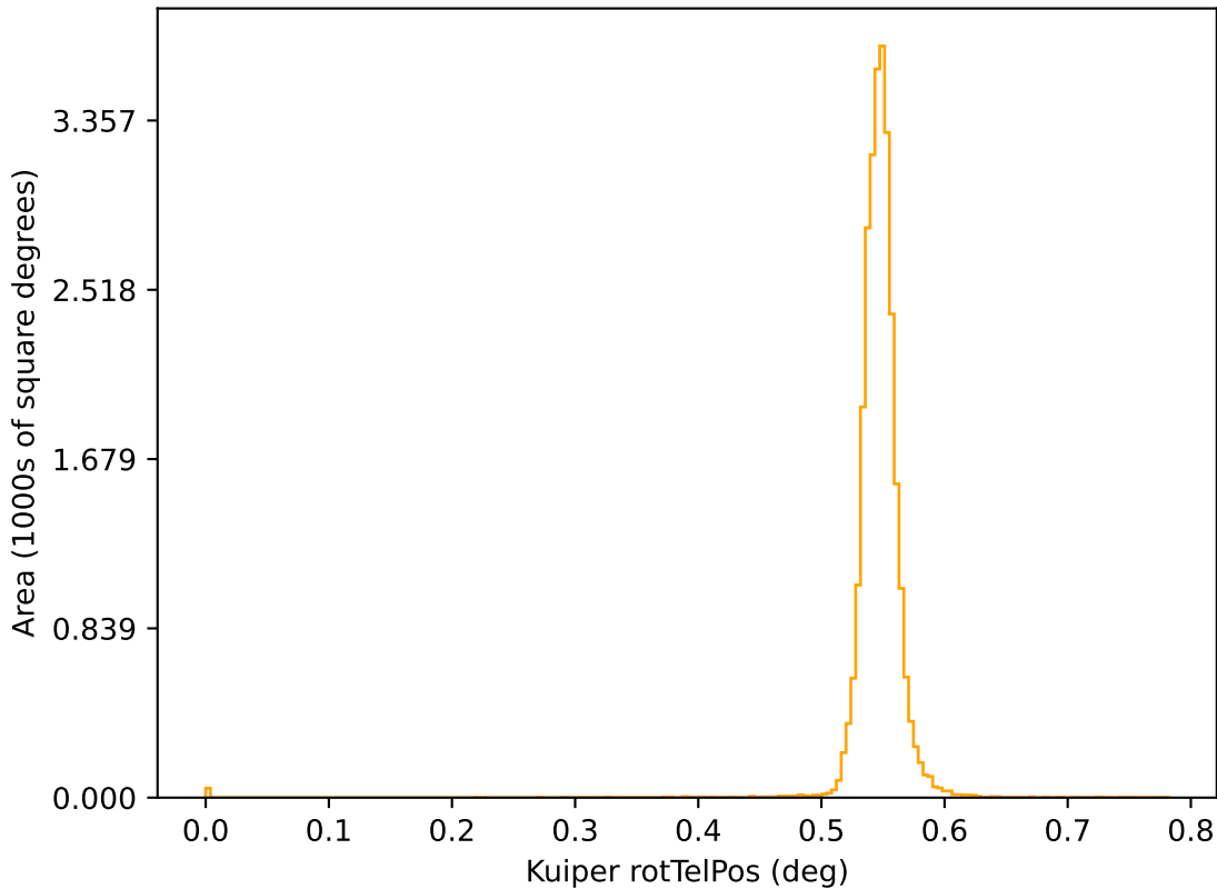
too_elab_r64_d2_ugrizy_v3.4_10yrs r: Kuiper rotTelPos
