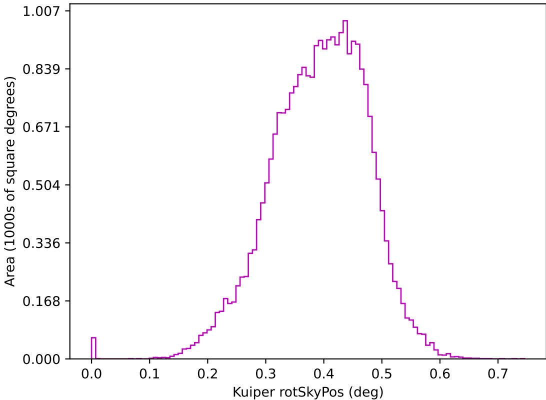
too_elab_r64_d2_ugrizy_v3.4_10yrs z: Kuiper rotSkyPos
