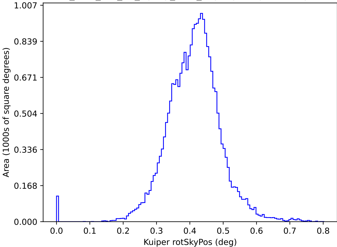
too_elab_r64_d2_ugrizy_v3.4_10yrs y: Kuiper rotSkyPos
