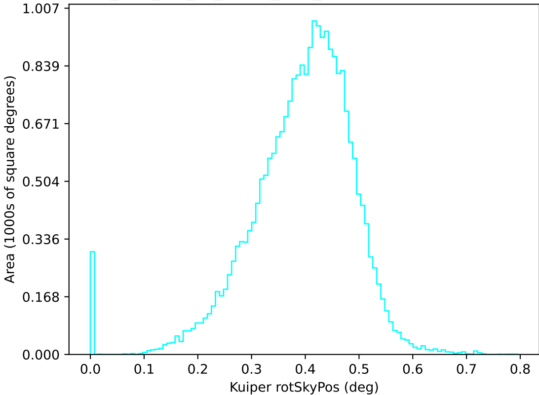
too_elab_r64_d2_ugrizy_v3.4_10yrs u: Kuiper rotSkyPos
