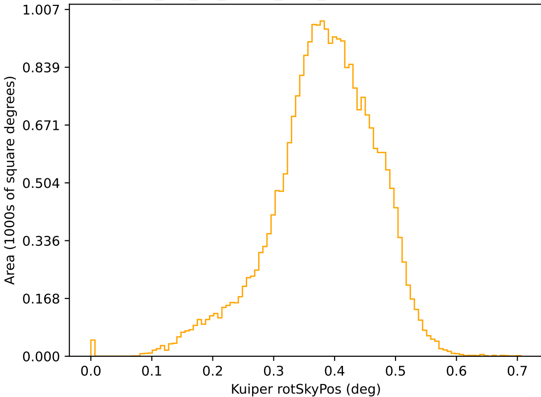
too_elab_r64_d2_ugrizy_v3.4_10yrs r: Kuiper rotSkyPos
