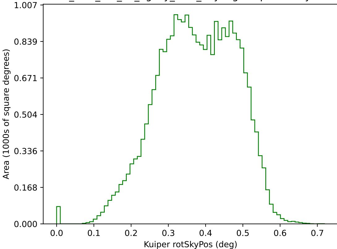
too_elab_r64_d2_ugrizy_v3.4_10yrs g: Kuiper rotSkyPos
