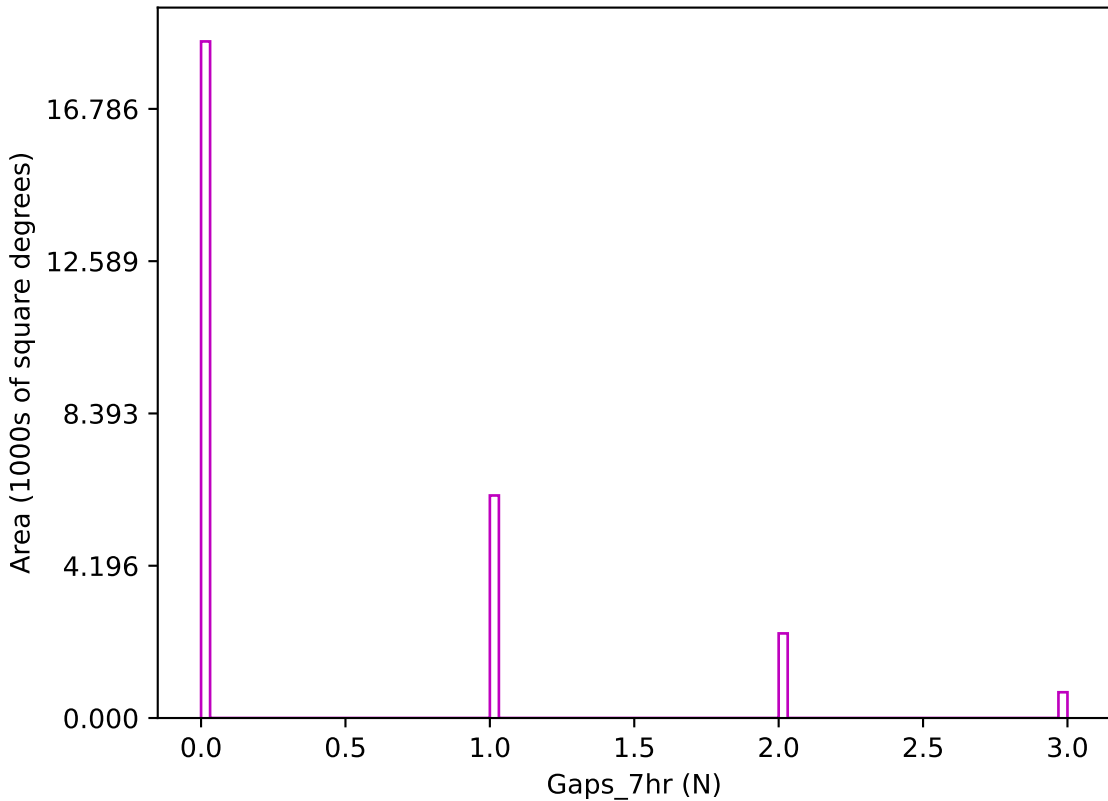
too_elab_r64_d2_ugrizy_v3.4_10yrs z band: Gaps_7hr
