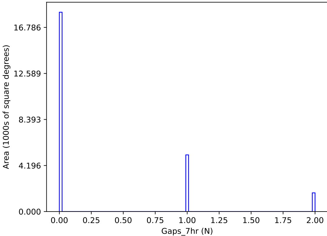
too_elab_r64_d2_ugrizy_v3.4_10yrs y band: Gaps_7hr
