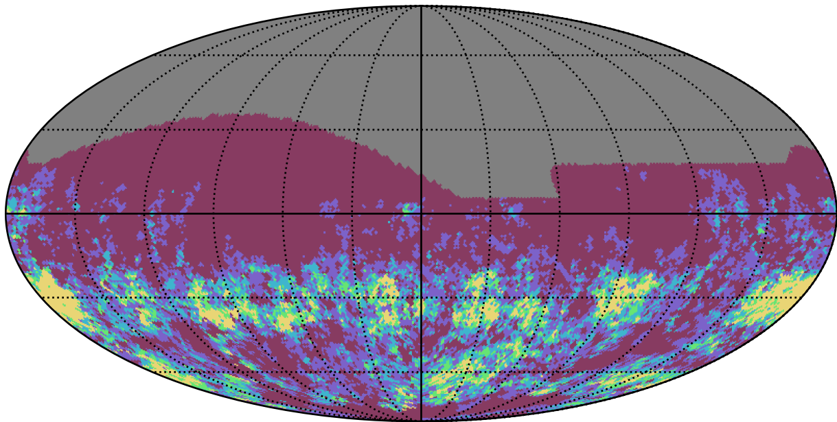
too_elab_r64_d2_ugrizy_v3.4_10yrs r band: Gaps_7hr
