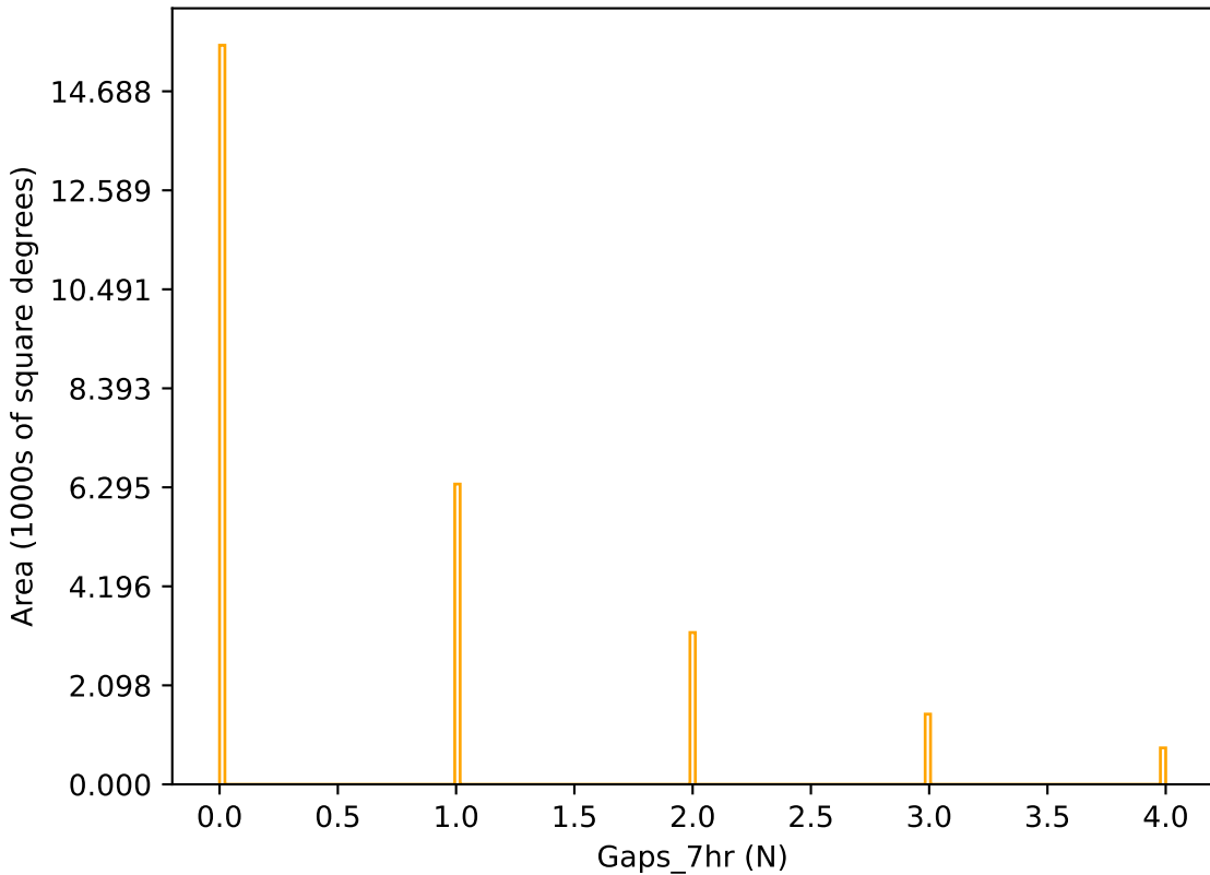
too_elab_r64_d2_ugrizy_v3.4_10yrs r band: Gaps_7hr
