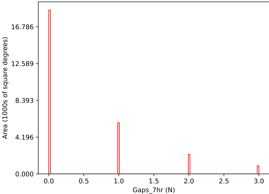
too_elab_r64_d2_ugrizy_v3.4_10yrs i band: Gaps_7hr
