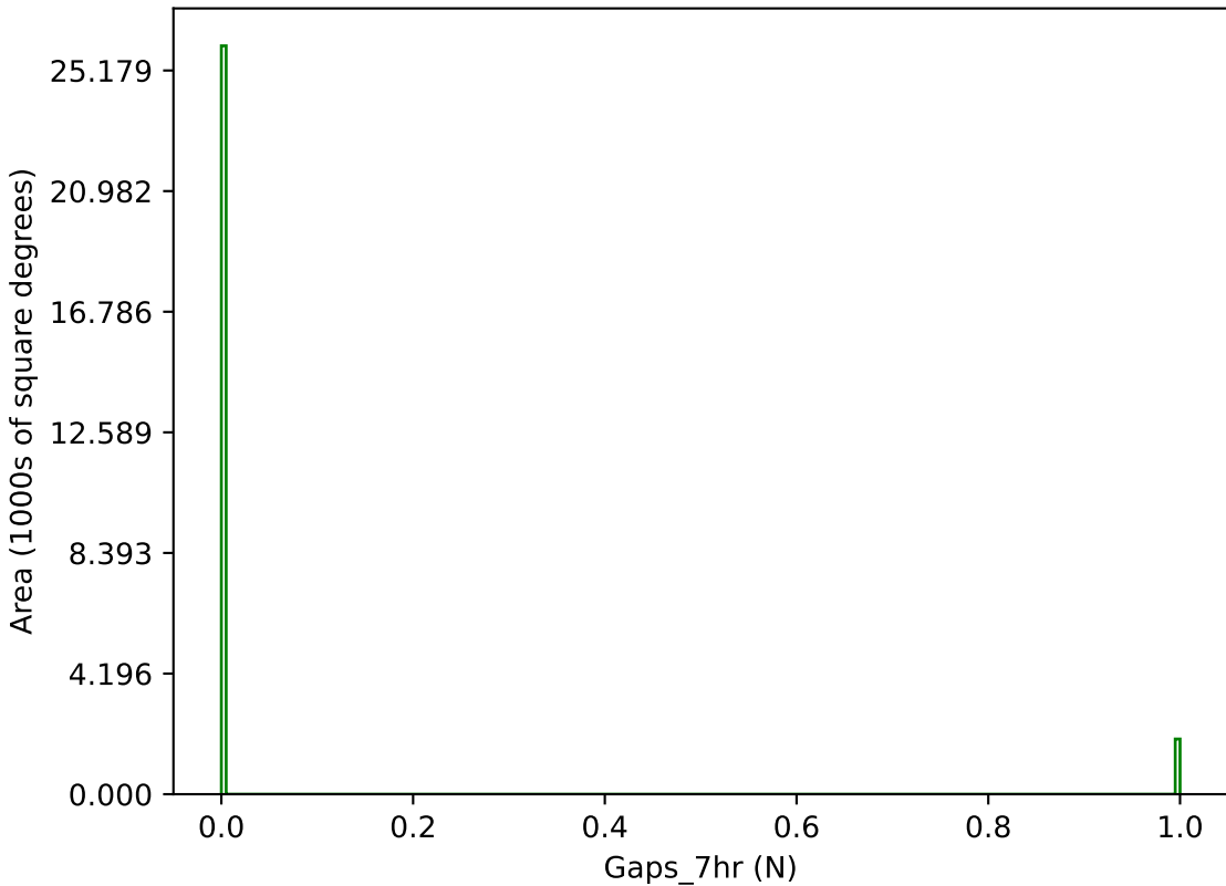
too_elab_r64_d2_ugrizy_v3.4_10yrs g band: Gaps_7hr
