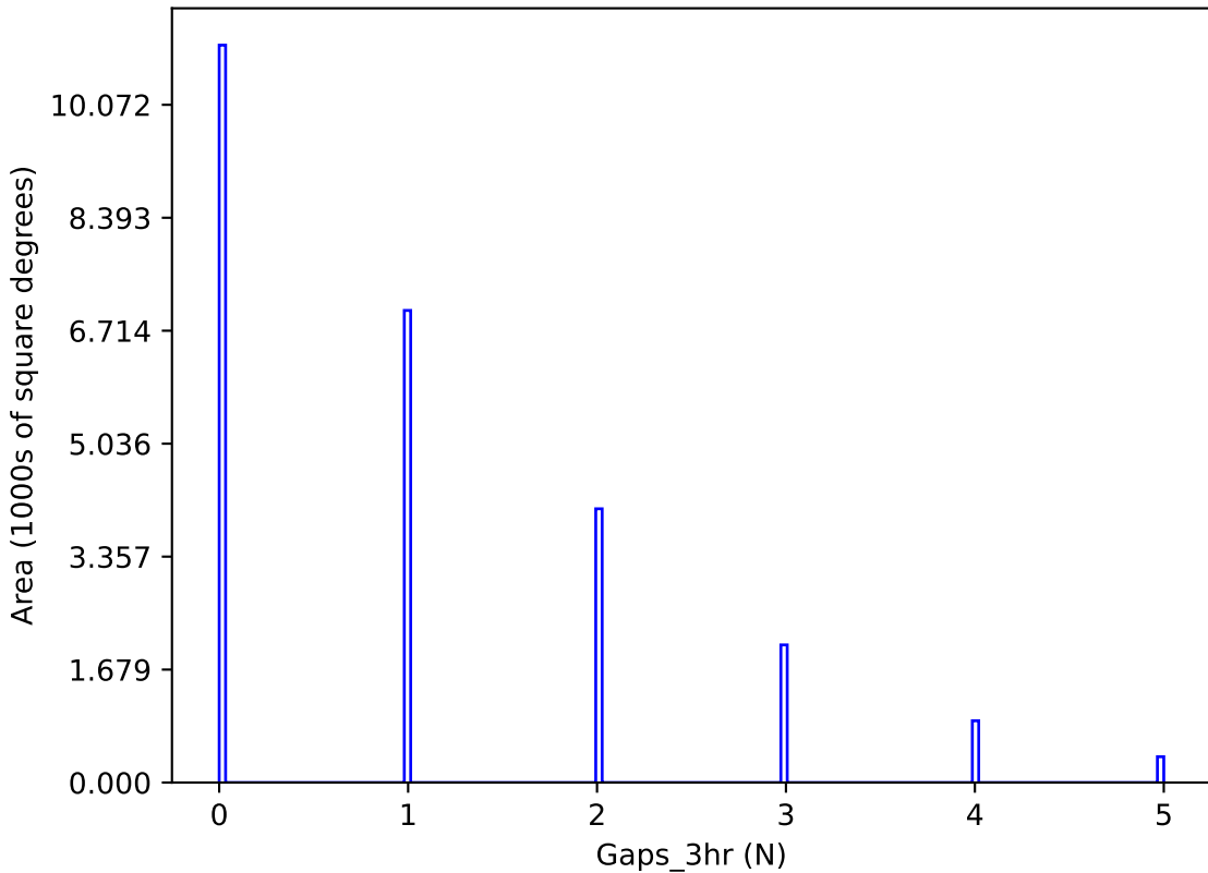
too_elab_r64_d2_ugrizy_v3.4_10yrs y band: Gaps_3hr
