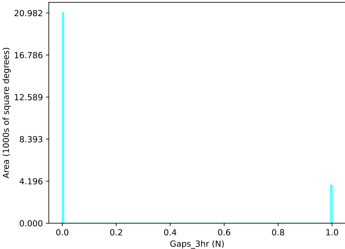
too_elab_r64_d2_ugrizy_v3.4_10yrs u band: Gaps_3hr
