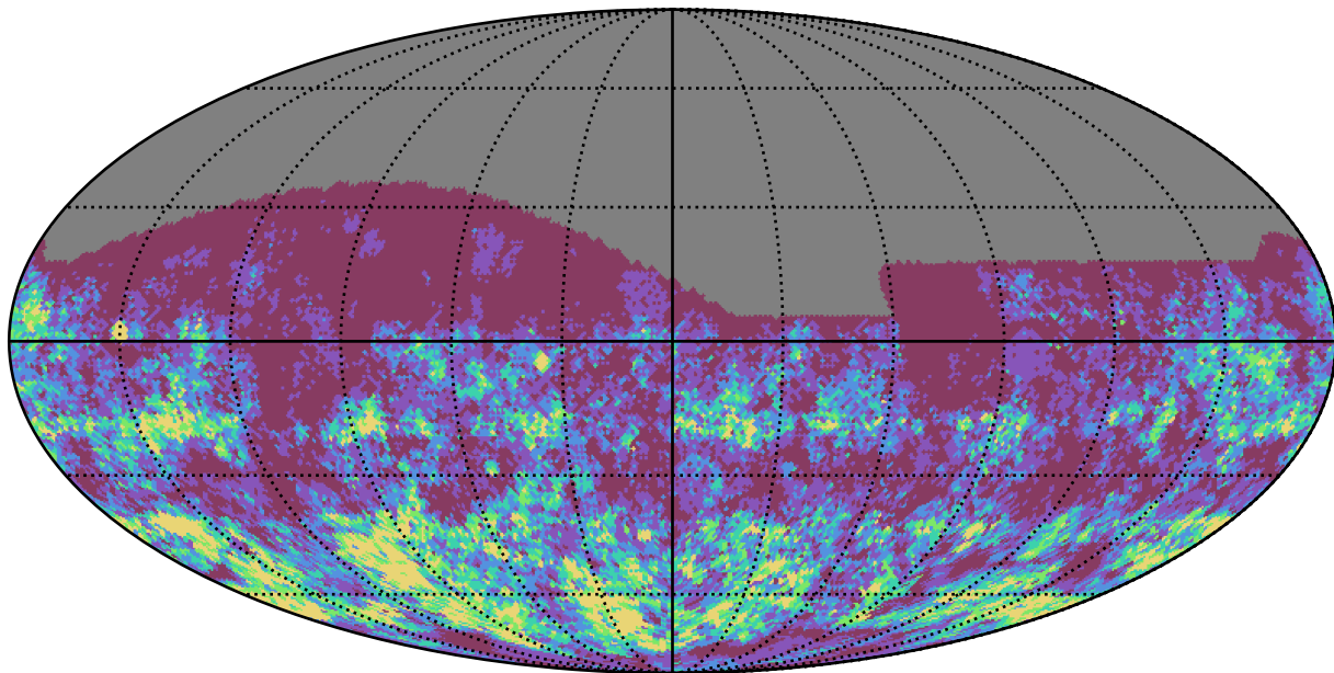
too_elab_r64_d2_ugrizy_v3.4_10yrs r band: Gaps_3hr
