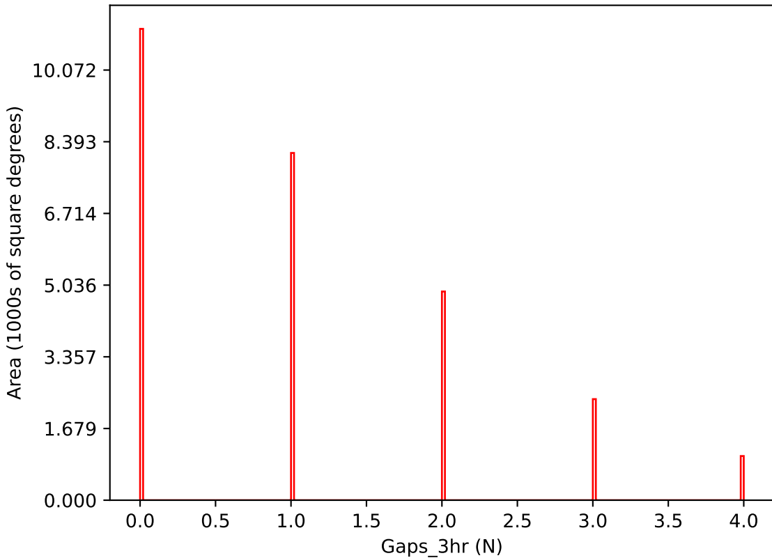
too_elab_r64_d2_ugrizy_v3.4_10yrs i band: Gaps_3hr
