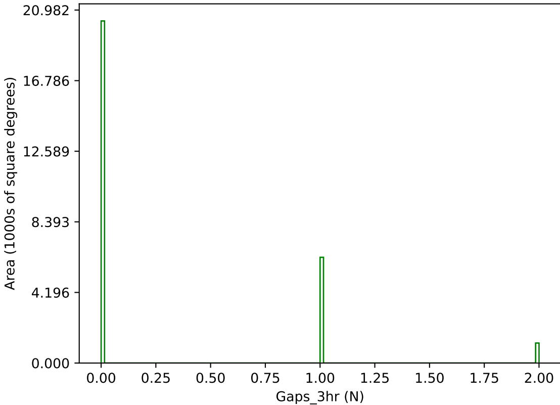
too_elab_r64_d2_ugrizy_v3.4_10yrs g band: Gaps_3hr
