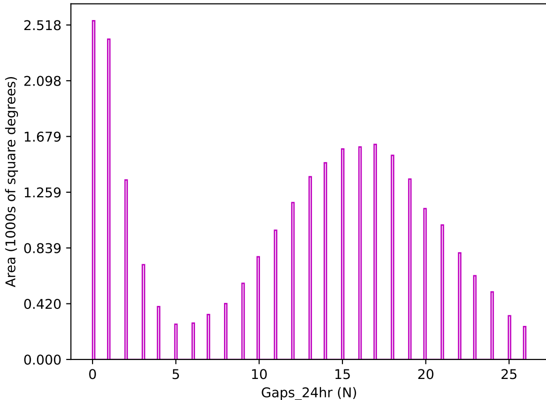
too_elab_r64_d2_ugrizy_v3.4_10yrs z band: Gaps_24hr
