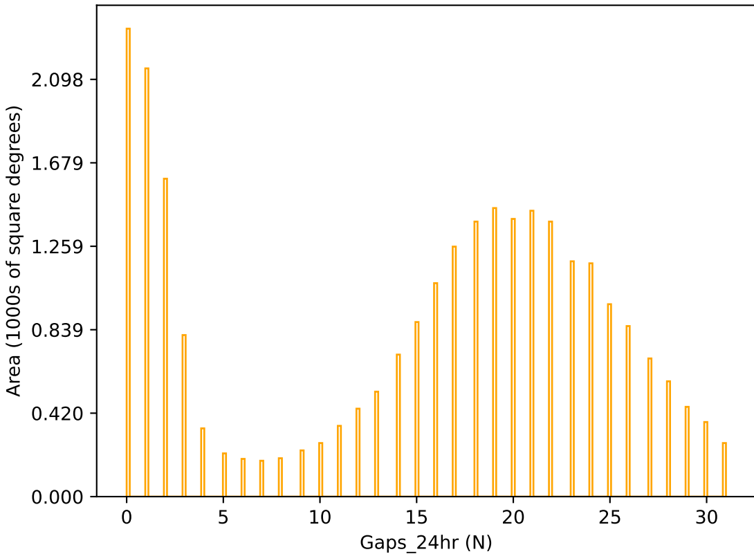
too_elab_r64_d2_ugrizy_v3.4_10yrs r band: Gaps_24hr
