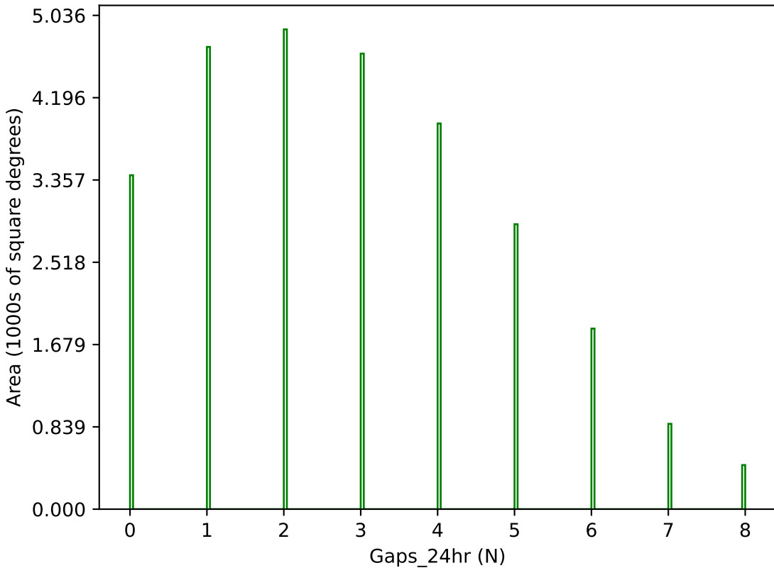
too_elab_r64_d2_ugrizy_v3.4_10yrs g band: Gaps_24hr
