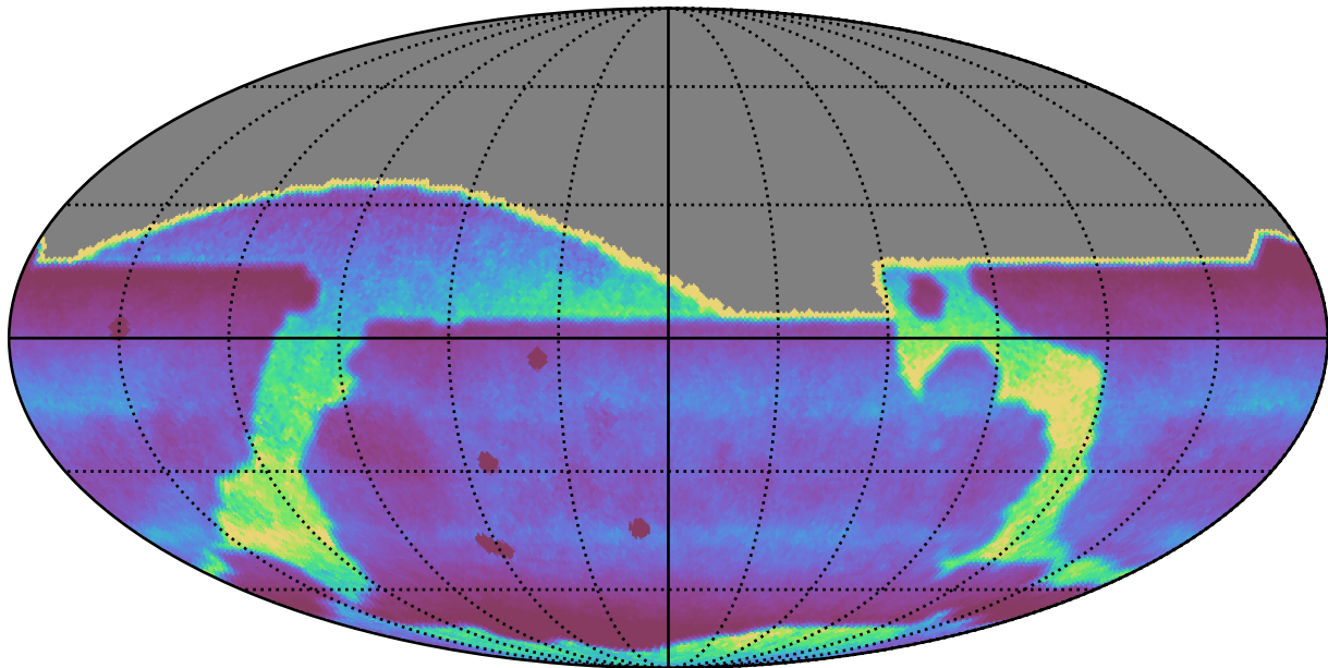
too_elab_r64_d2_ugrizy_v3.4_10yrs : DCRprecision
