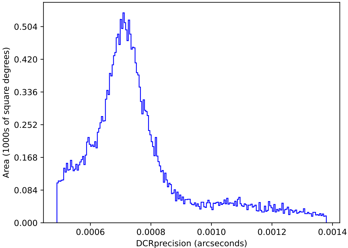
too_elab_r64_d2_ugrizy_v3.4_10yrs : DCRprecision
