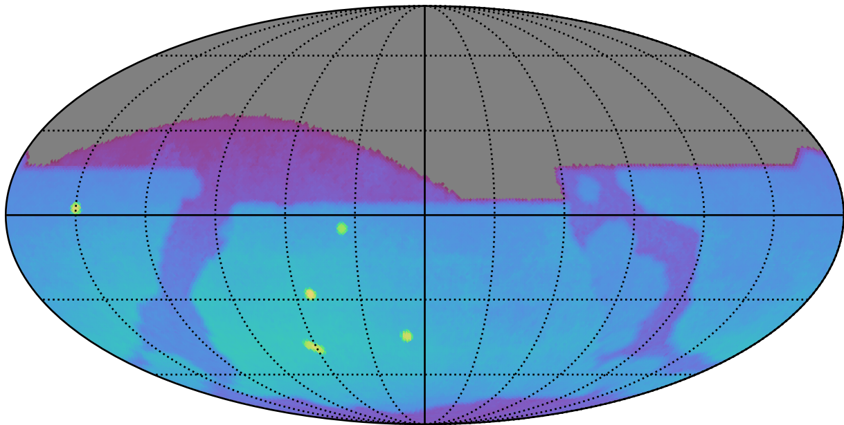
too_elab_r64_d2_ugrizy_v3.4_10yrs : Brown Dwarf, L7
