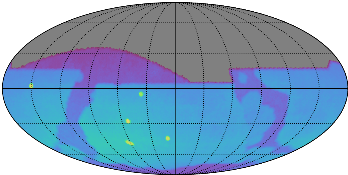
too_elab_r64_d2_ugrizy_v3.4_10yrs : Brown Dwarf, L4
