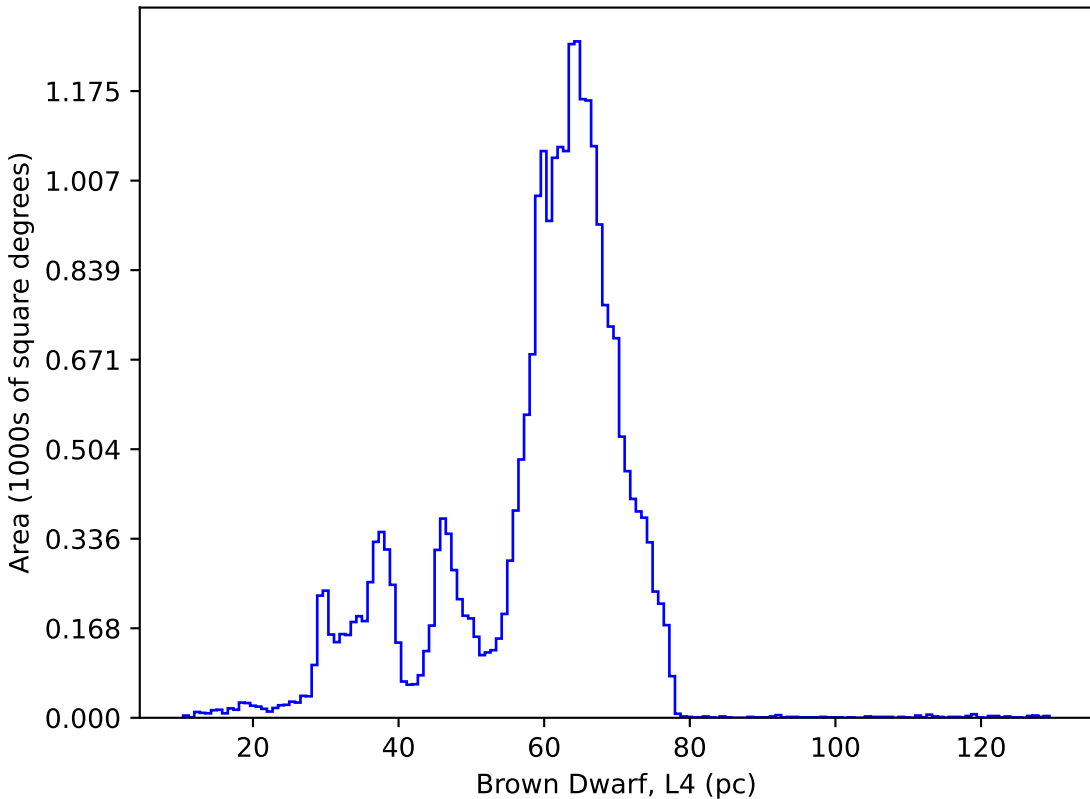
too_elab_r64_d2_ugrizy_v3.4_10yrs : Brown Dwarf, L4
