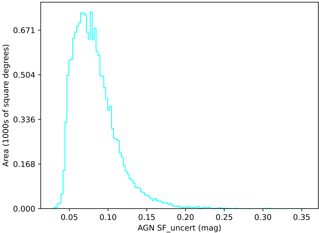
too_elab_r64_d2_ugrizy_v3.4_10yrs u band: AGN SF_uncert
