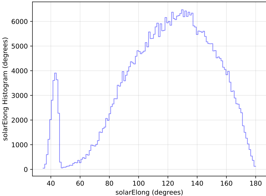
too_elab_r64_d2_ugrizy_v3.4_10yrs WFD z band: solarElong Histogram
