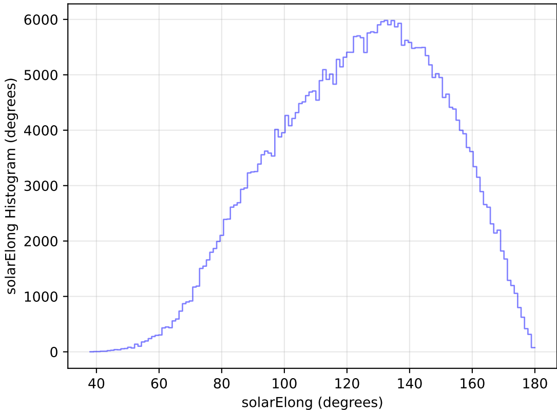
too_elab_r64_d2_ugrizy_v3.4_10yrs WFD y band: solarElong Histogram
